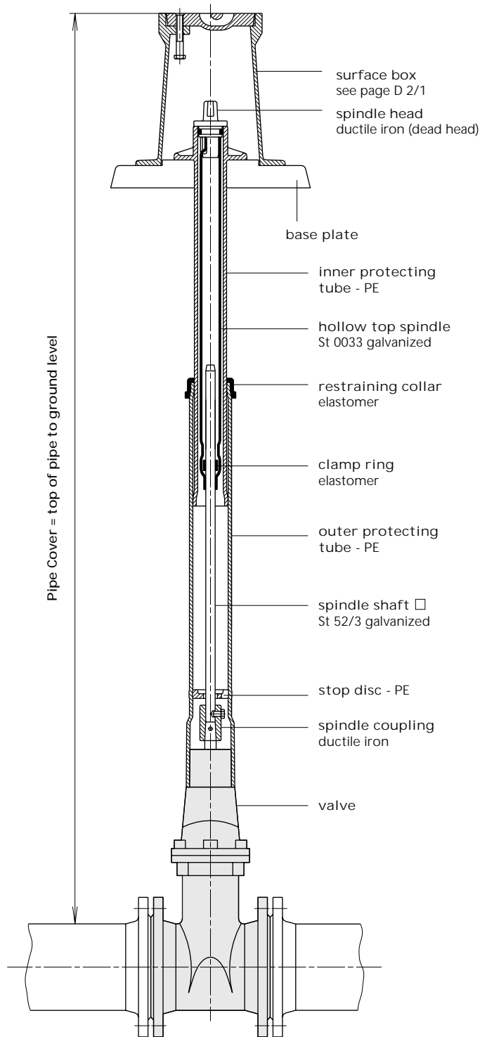
Illustration: telescopic Extension Spindle DN 250 - 500
